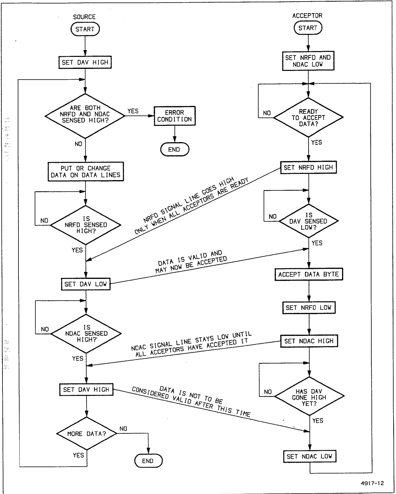
Figure 3-11. GPIB data flow diagram.
