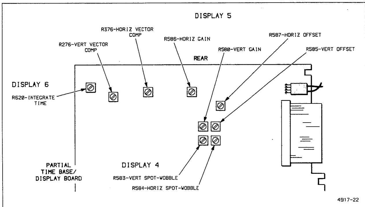
Figure 5-1. Adjustment locations for Displays 4 through 6.
