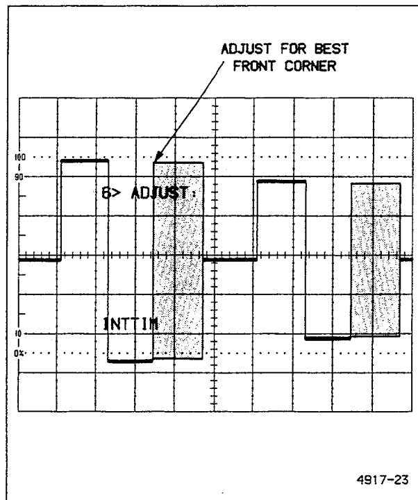
Figure 5-3. Display 6—Integrator Time adjustment pattern.
