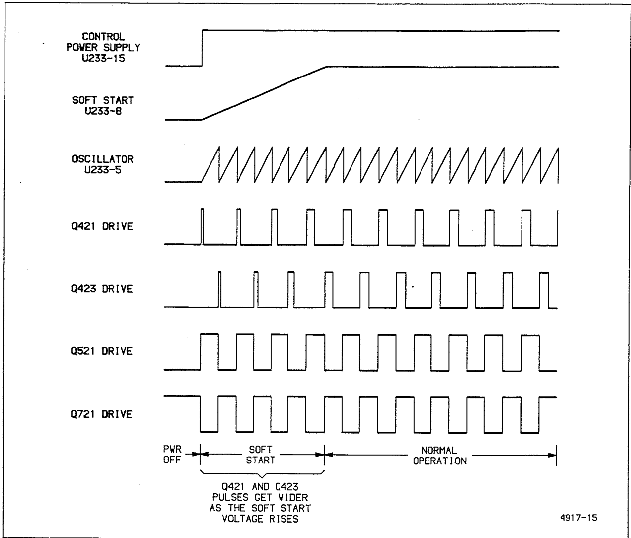
Figure 3-16. PWM switching waveforms.
