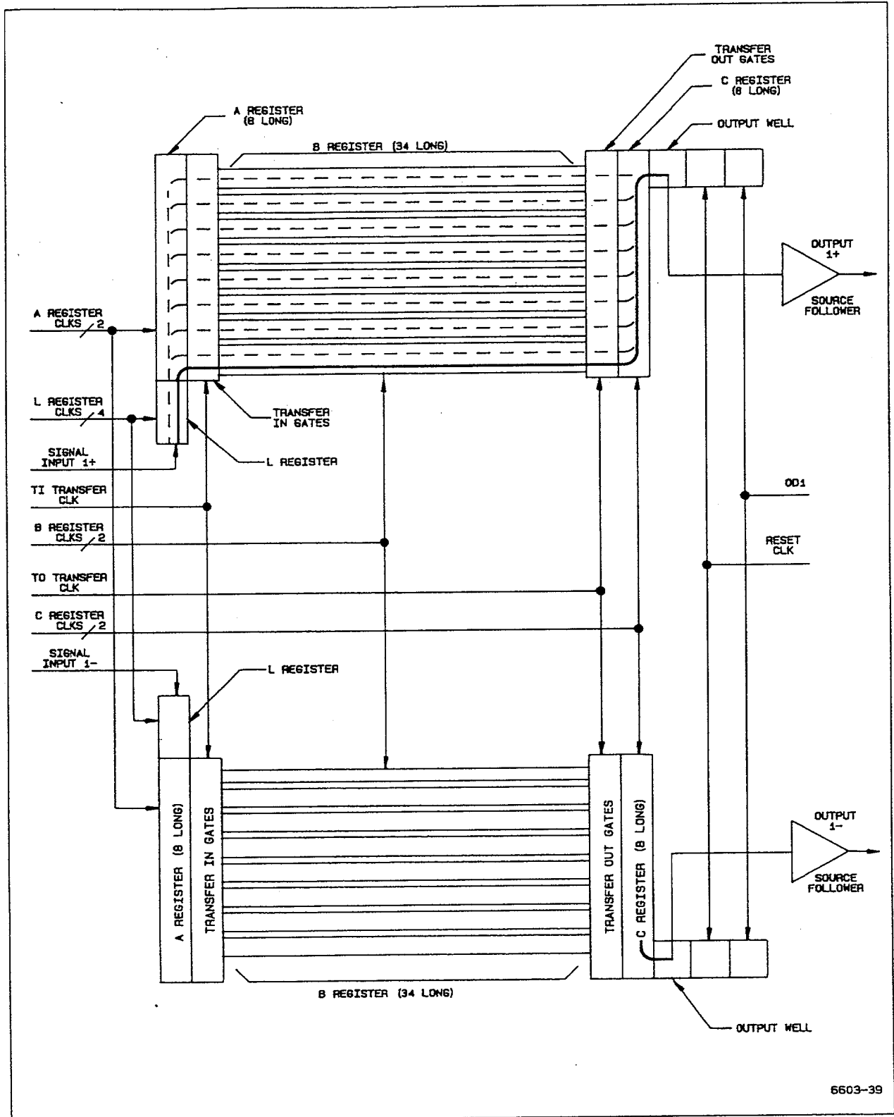
Figure 3-5. Simplified CCD architecture.
