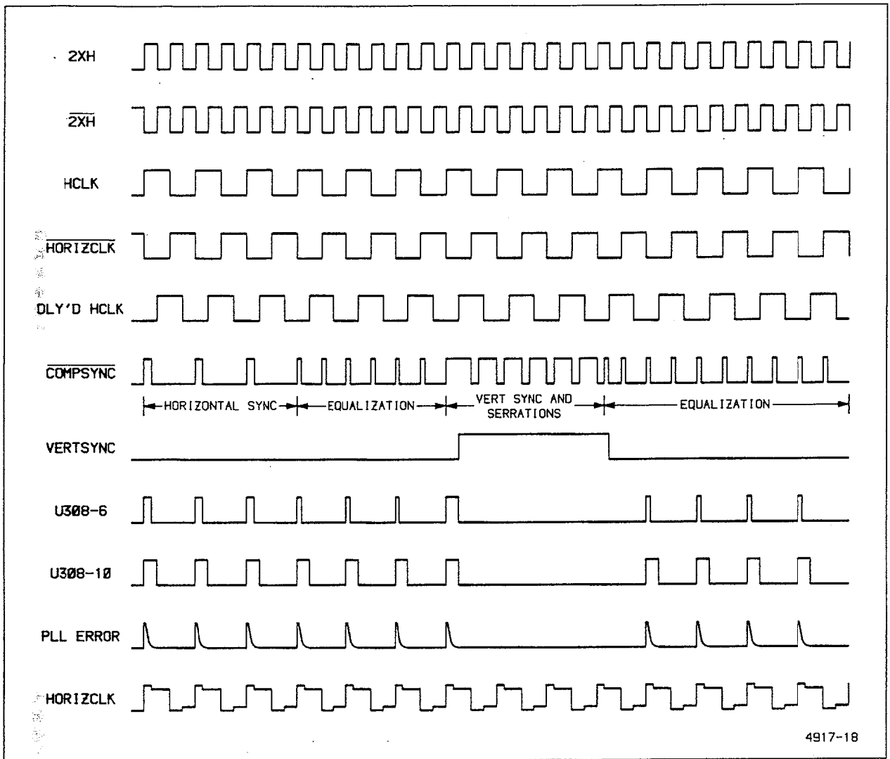
Figure 3-13. Video Option waveforms.
