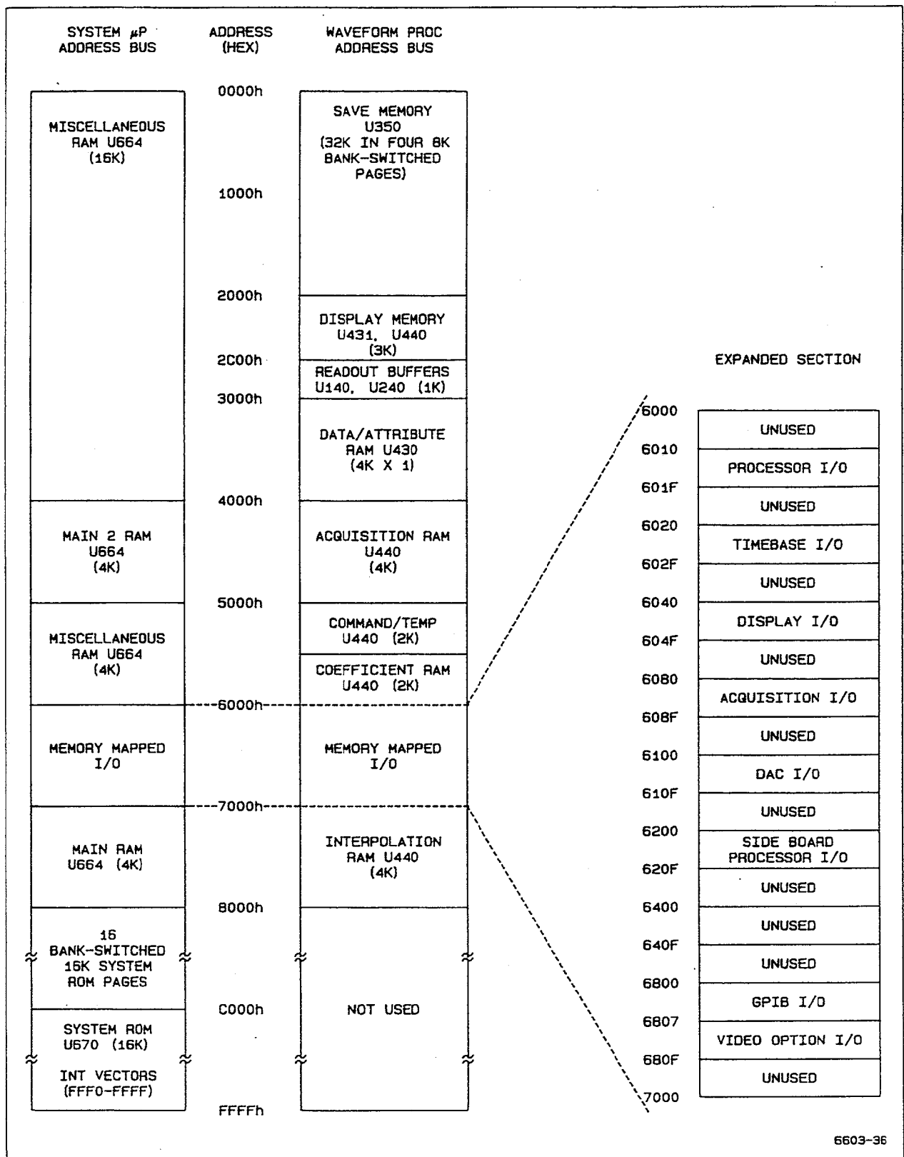
Figure 3-2. Simplified Memory Map
