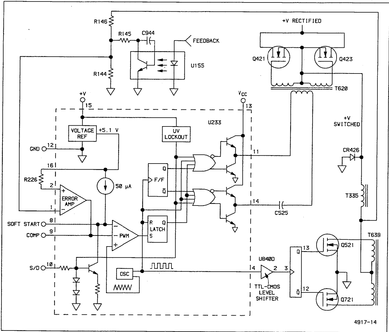
Figure 3-15. PWM Regulator and Inverter.
