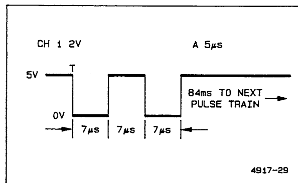
Figure 6-9. Front Panel \mu P diagnostics test.
