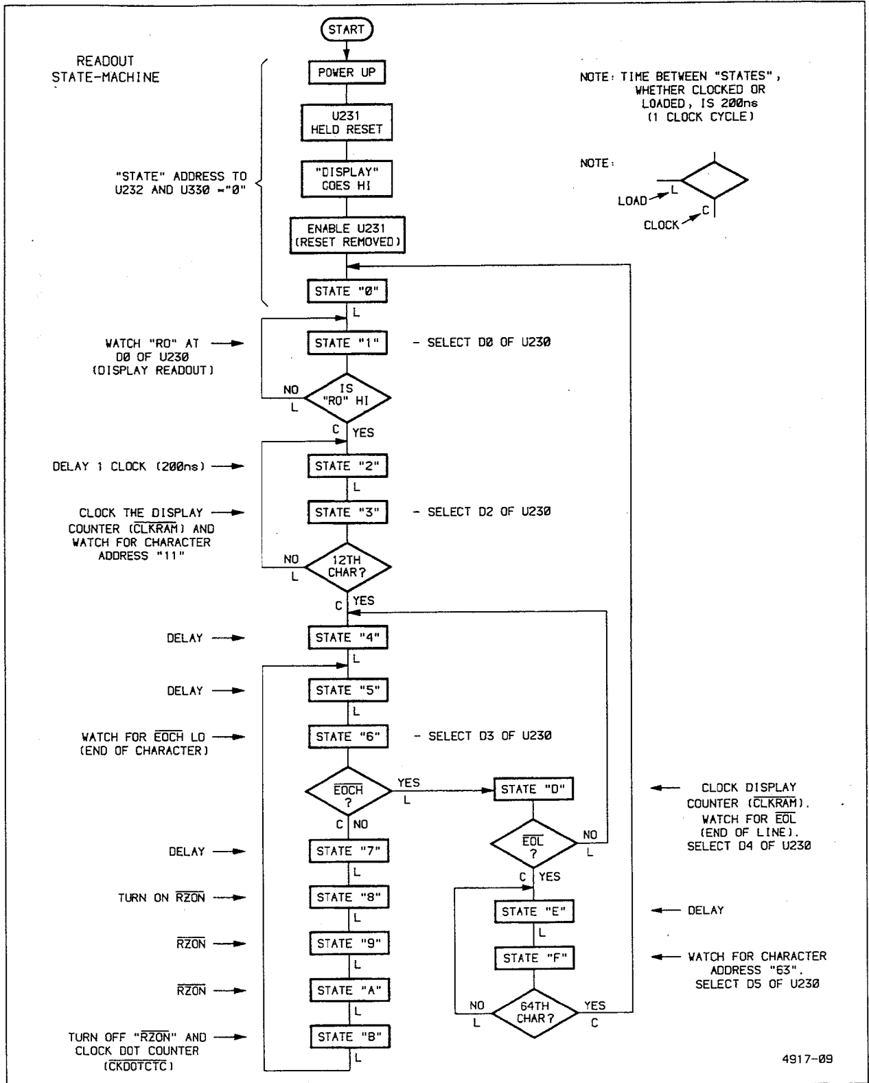
Figure 3-8. Readout State Machine flow chart.
