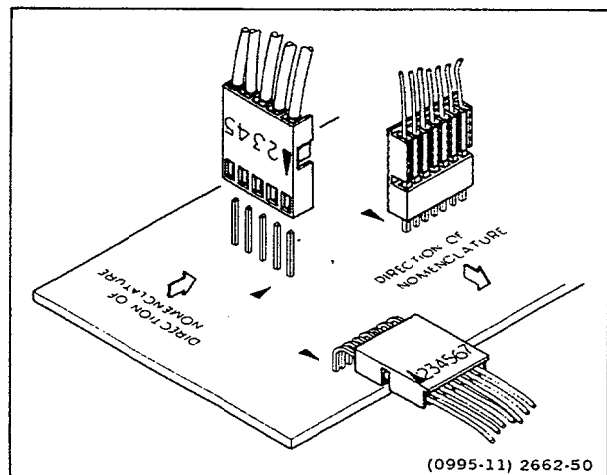
Figure 6-1. Multipin connector.
