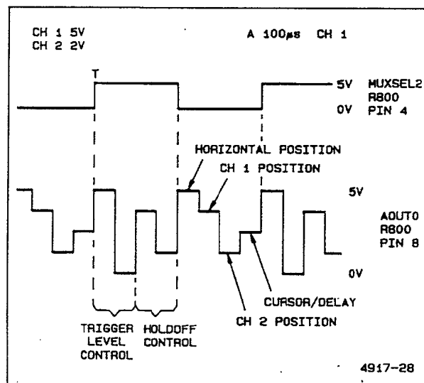
Figure 5-7. Mux Test waveforms.
