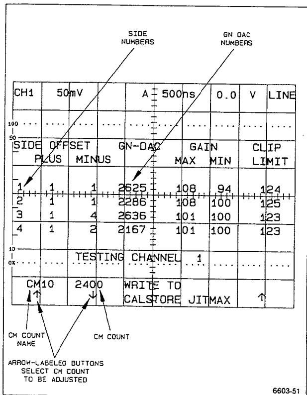
Figure 5-5. CCD counts display and CM adjustment menu.
