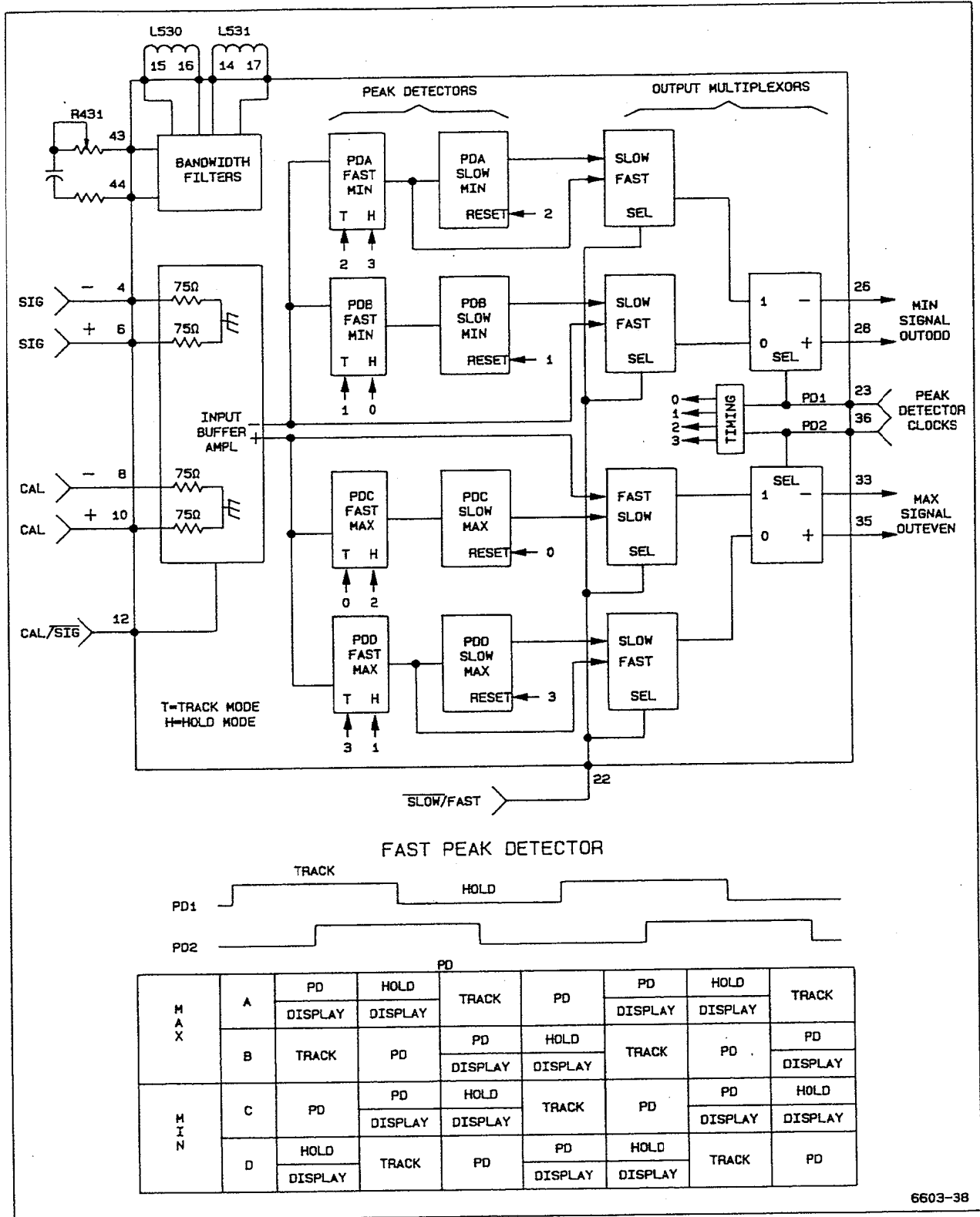
Figure 3-4. Simplified Peak Detector block diagram.
