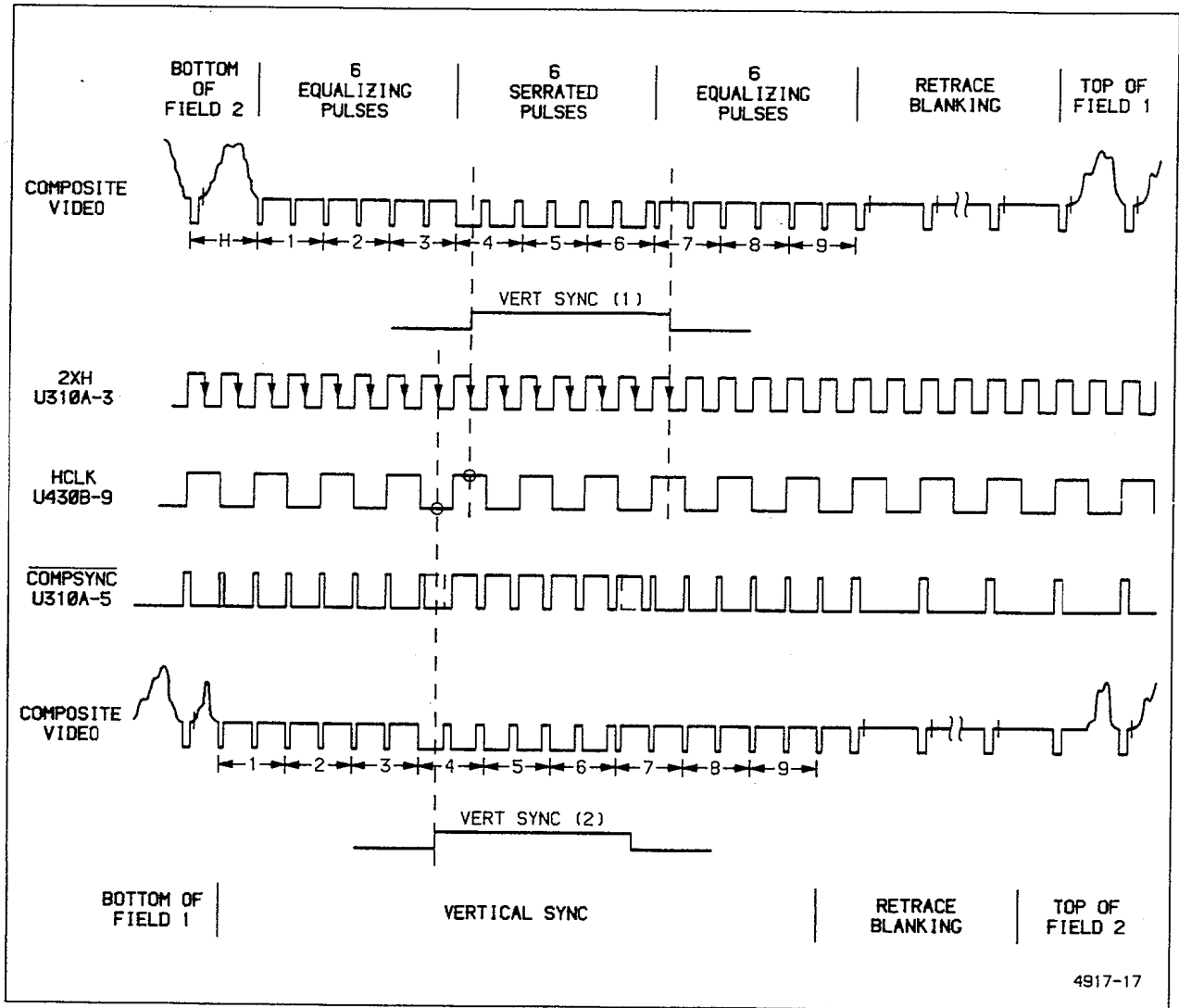
Figure 3-14. Video Option field-sync identification.
