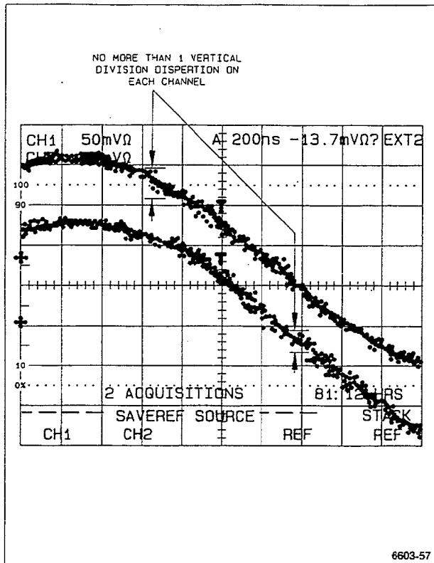
Figure 5-11. Checking sample dispersion.
