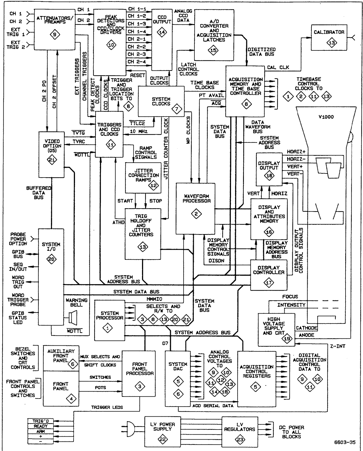
Figure 3-1. Simplified block diagram.
