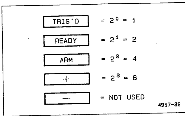
Figure 6-4. Trigger LED binary coding for diagnostic tests.
