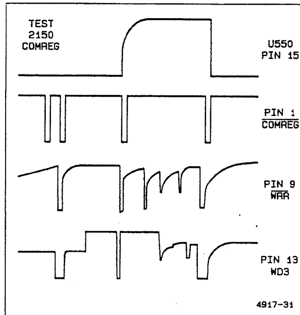
Figure 6-8. Typical Register test waveforms.
