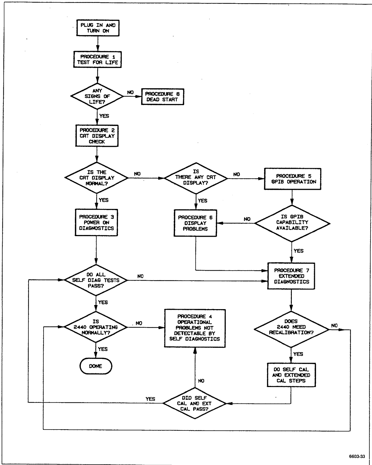
Figure 6-6. Initial troubleshooting chart.
