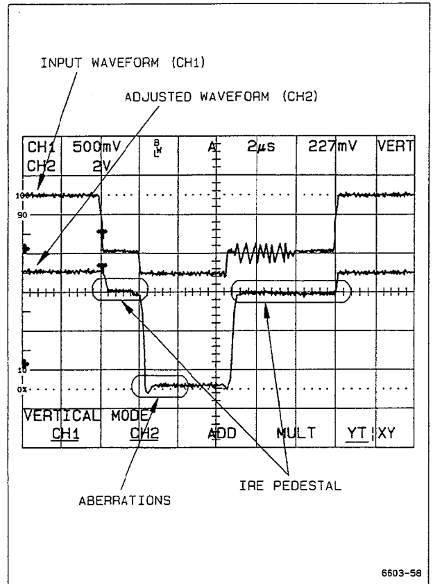
Figure 5.12 Input and output (after adjustment) waveforms.
