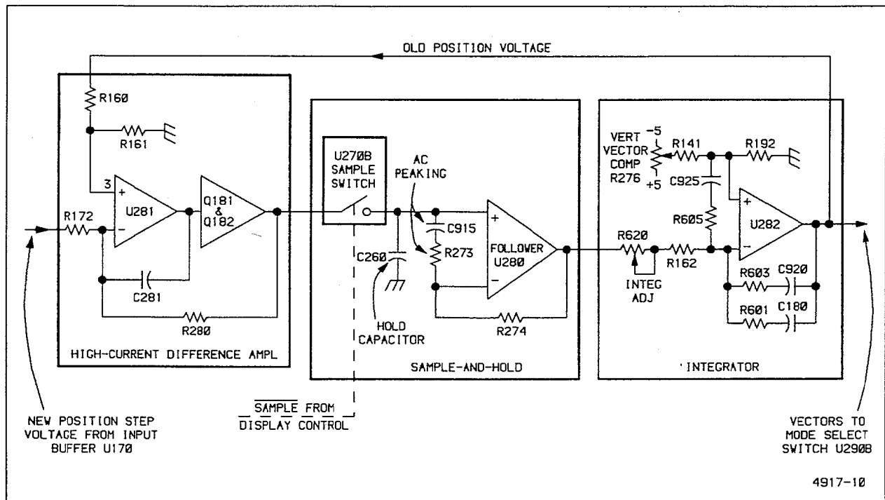
Figure 3-9. Vertical Vector Generator.
