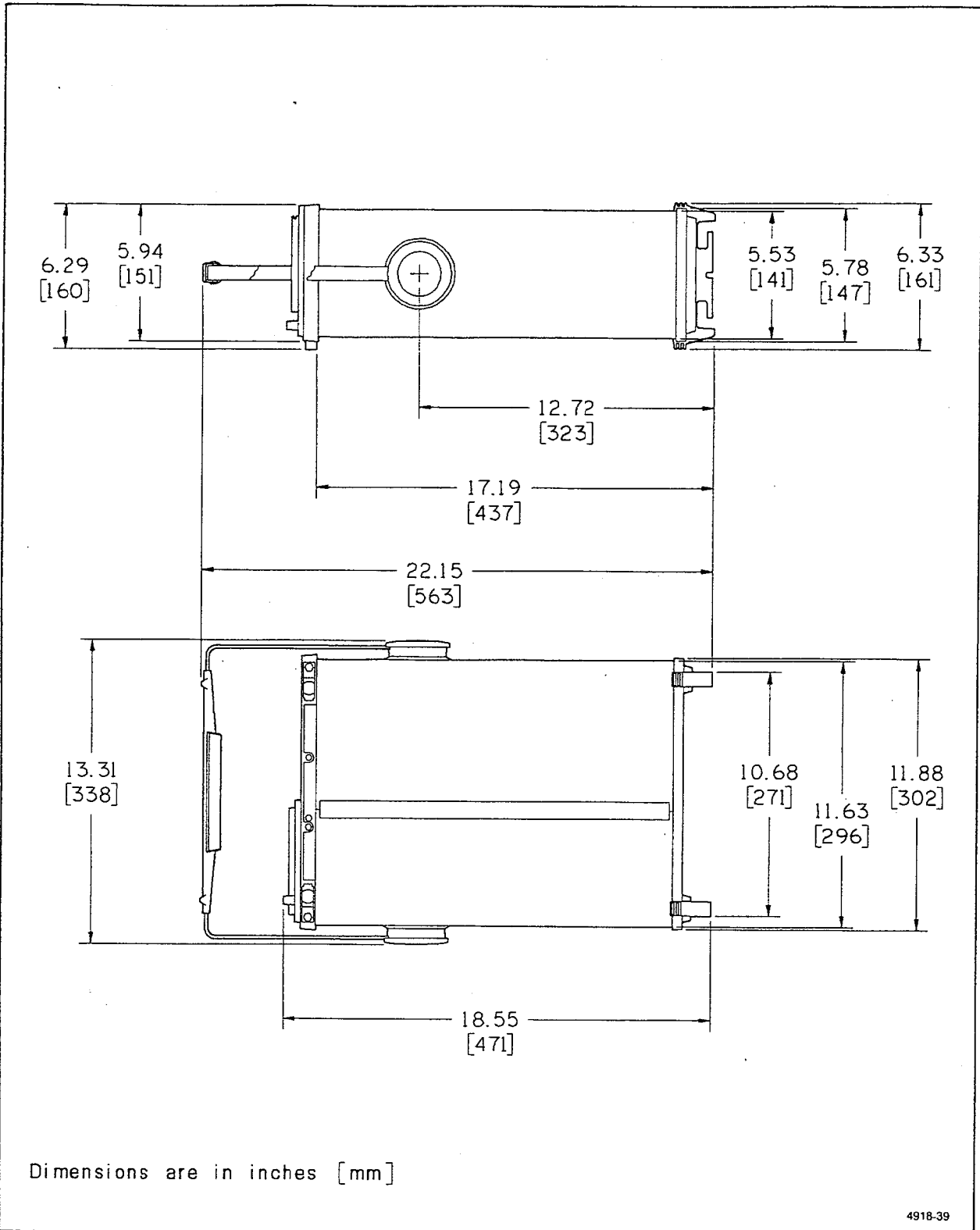
Figure 1-1. Dimensional drawing.
