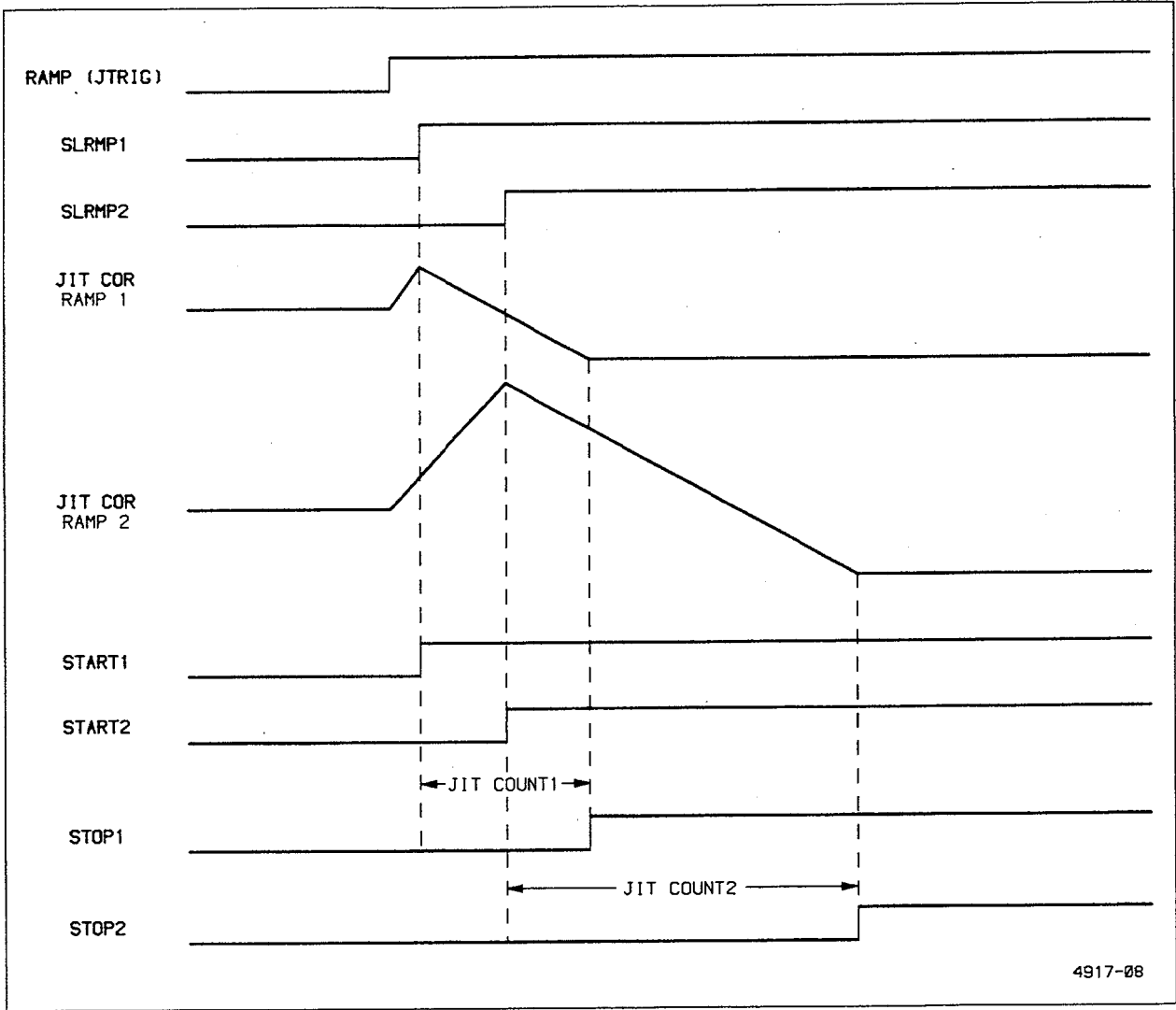
Figure 3-7. Jitter Correction waveforms.
