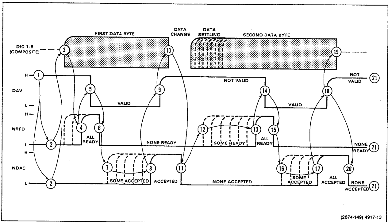
Figure 3-12. GPIB three-wire handshake state diagram.
