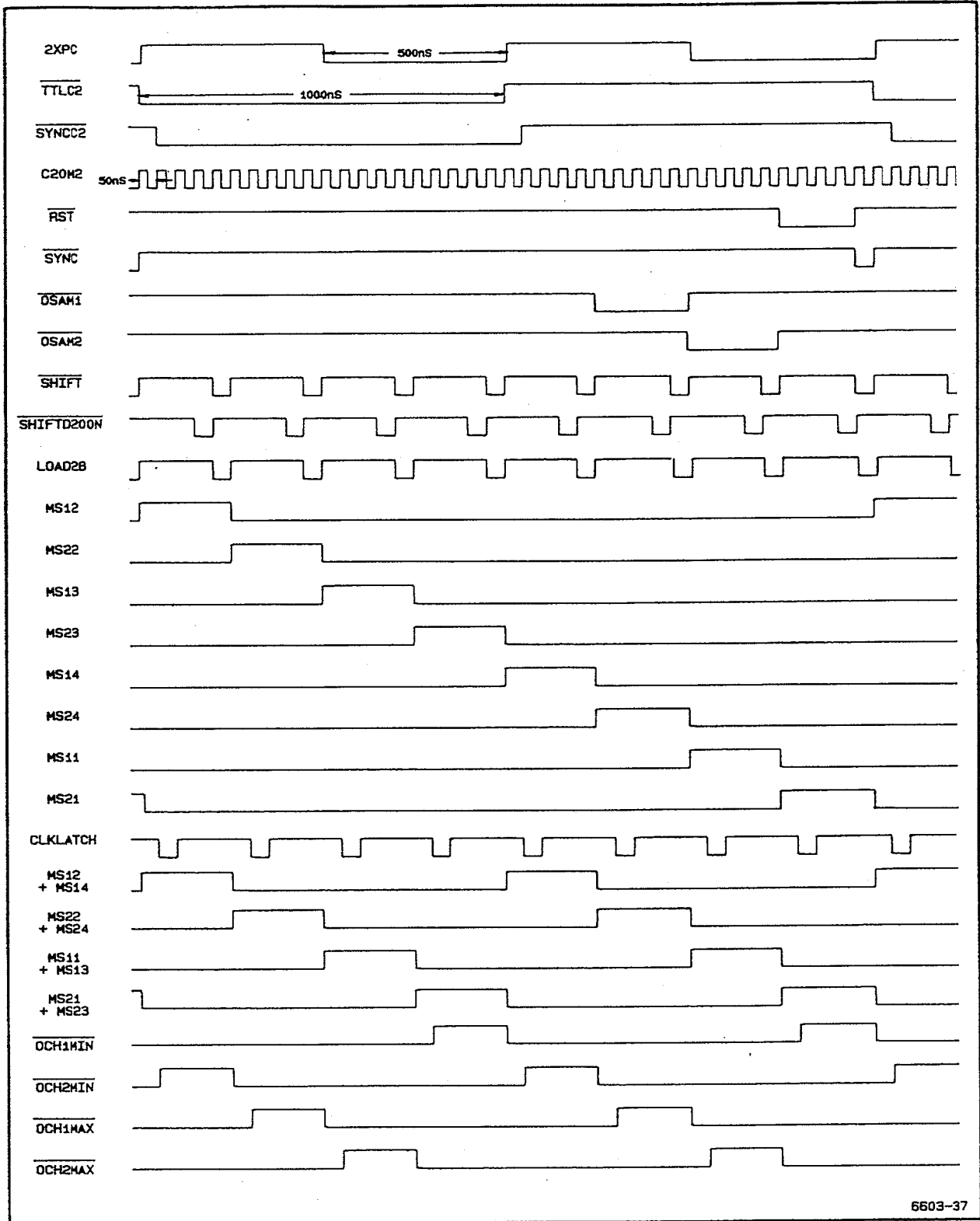
Figure 3-3. System Clock waveforms.
