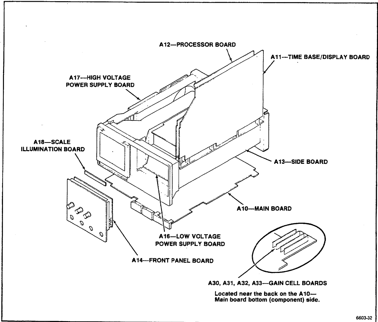
Figure 6-2. Circuit Board Location.
