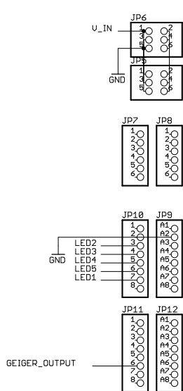
Arduino connectors
